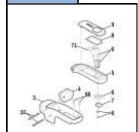
ASSEMBLY 2
