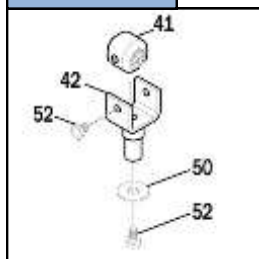
ASSEMBLY 3
